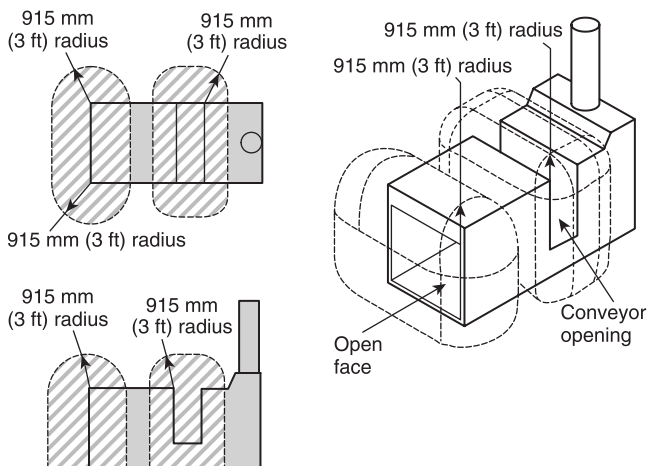
▲ FIGURE 43.1.4.4.2(a) Class I, Division 2; Zone 2; Class II, Division 2; or Zone 22 Locations Adjacent to an Open-Face or Open-Front Spray Booth or Spray Room. [33:Figure 6.5.2(a)]
