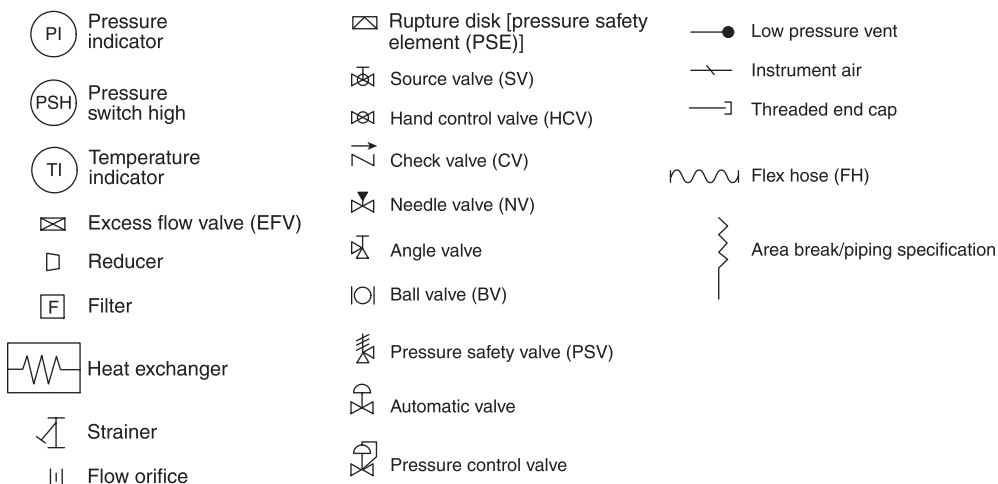
FIGURE A.3.3.283.1(a) Symbol Legend for Figure A.3.3.274.1(b) through Figure A.3.3.274.1(f). [55:Figure A.3.3.95.1(a)]
