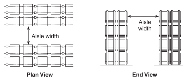
FIGURE A.3.3.11 Illustration of Aisle Width. [13:Figure A.3.3.4]
