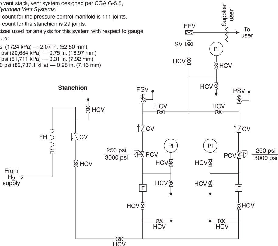
FIGURE A.3.3.283.1(d) Typical Trailer Discharge Stanchion and Pressure Control Manifold. [55:Figure A.3.3.95.9.1(d)]
