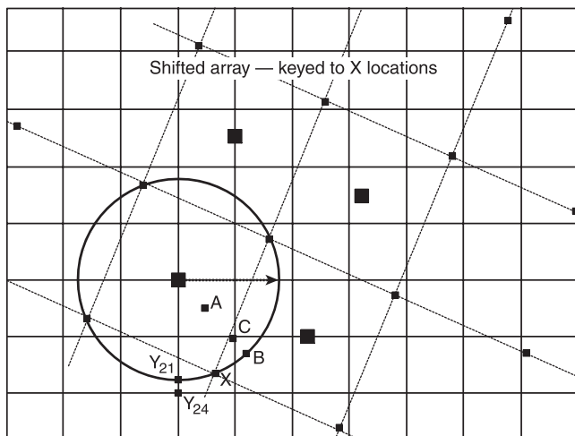
▲ FIGURE A.13.7.4.3.4.2(3)(b) Shifted Smoke Detection Grid to Optimize Detection for Deep Beam Effects. [72: Figure A.17.7.4.2.4.2(3)(b)]
