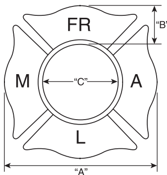
FIGURE C.1.2.4 Dimensions for Firefighter Safety Building Marking System Signs.
