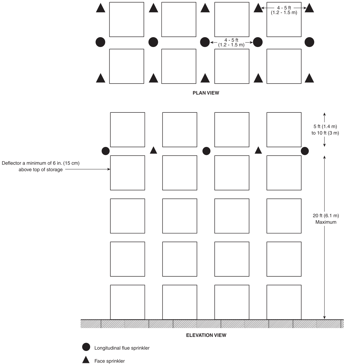
FIGURE 66.16.6.1(b) Double-Row Rack Sprinkler Layout for Design Scheme “F.” (Multiple row racks shall extend the same sprinkler pattern through the rack.) [30:Figure 16.6.6.1(b)]
