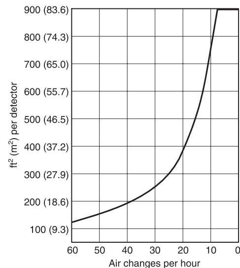
FIGURE 13.7.4.3.8.2.2 High Air Movement Areas (Not to Be Used for Under-Floor or Above-Ceiling Spaces). [72:Figure 17.7.7.3.3.2]
