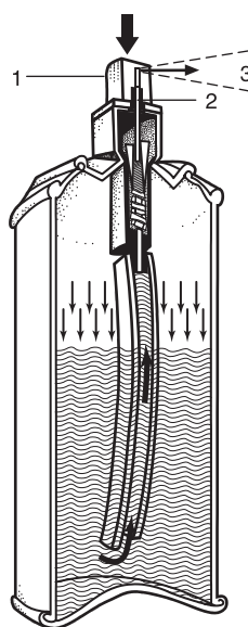
N FIGURE A.3.3.5 One Type of Aerosol Container (Cutaway View). When the plunger (1) is pressed, a hole in the valve (2) allows a pressurized mixture of product and propellant (3) to flow through the plunger's exit orifice. [Source: Fire Protection Handbook, 20th edition] [30B:Figure A.3.3.1] (FCC-HAZ)
