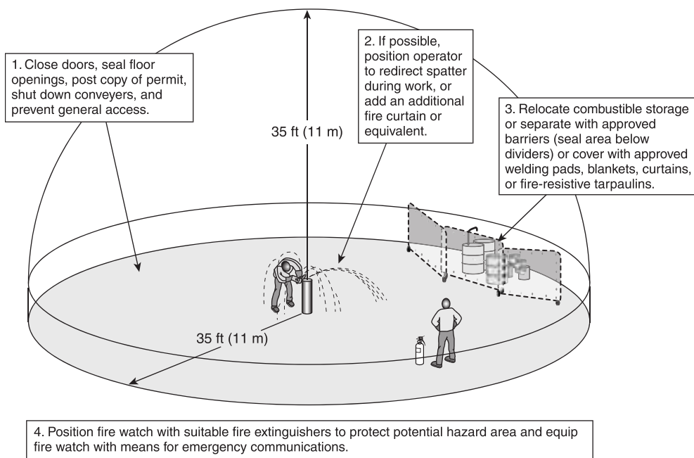
▲ FIGURE A.41.3.6.1(1)(a) The 35 Foot Rule Illustrated. [51B:Figure A.5.6.1(1)(a)]
