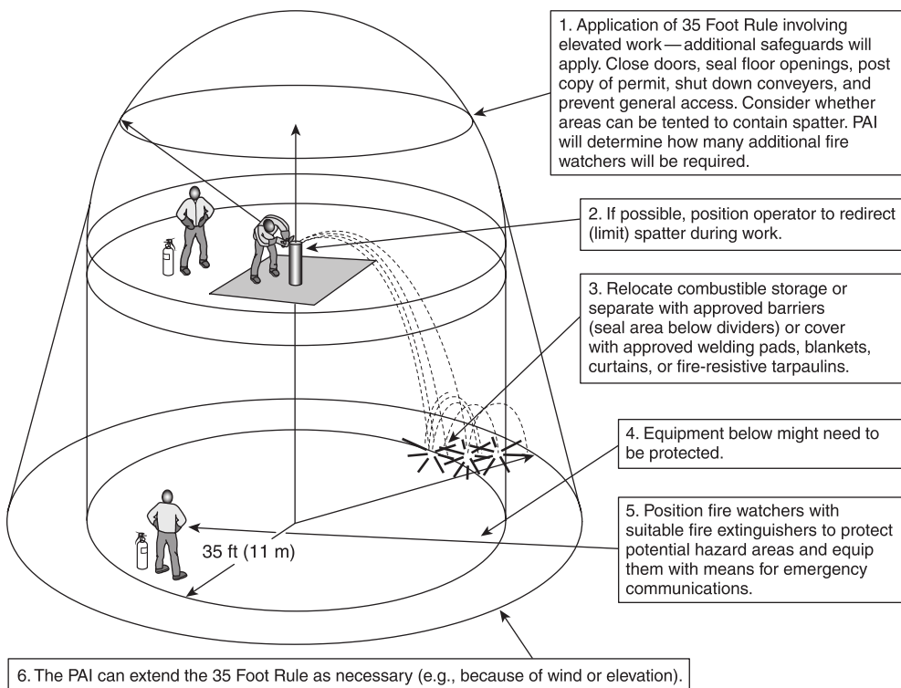
▲ FIGURE A.41.3.6.1(1)(b) Example of Where Multiple Fire Watches Are Needed. [51B:Figure A.5.6.1(1)(b)]
