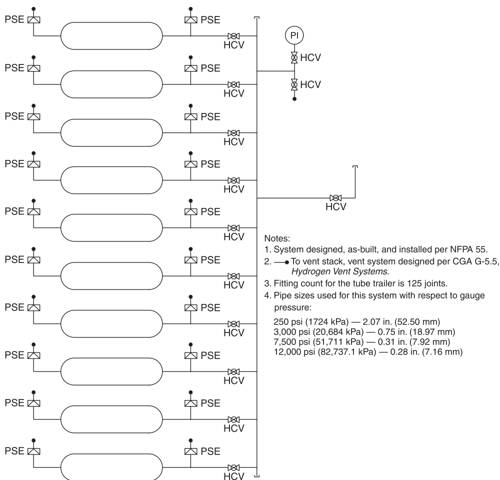
FIGURE A.3.3.283.1(b) Typical Tube Trailer. [55:Figure A.3.3.95.1(b)]
