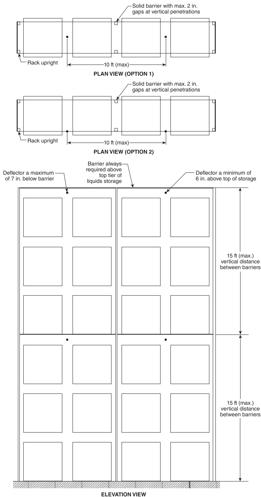
FIGURE 66.16.6.5.1(a) Single-Row Rack Sprinkler Layout for Design Scheme "E." [30:Figure 16.6.5.1(a)]
