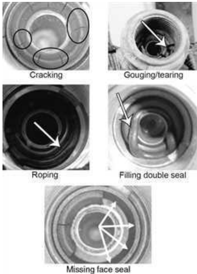
△ FIGURE A.69.4.2.2.7 Examples of Defects. [Figure 58:A.7.2.2.7]
