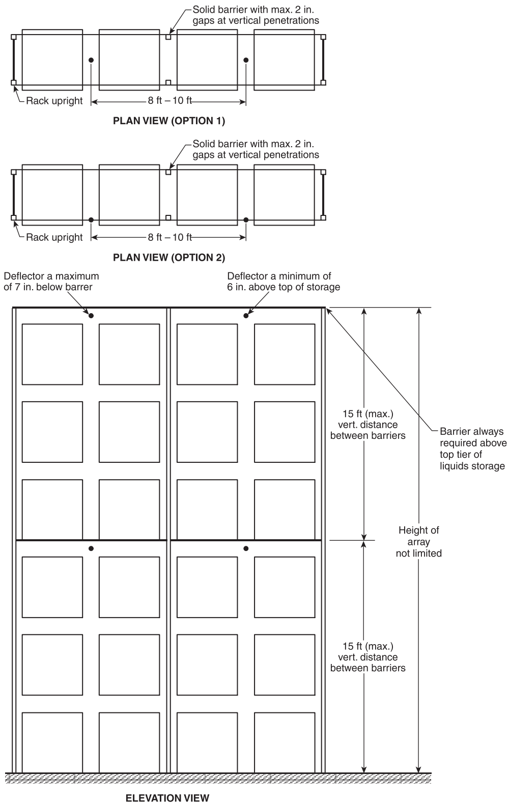
FIGURE 66.16.6.4.1(a) Single-Row Rack Sprinkler Layout for Fire Protection System Design Scheme "D." [30:Figure 16.6.4.1(a)]
