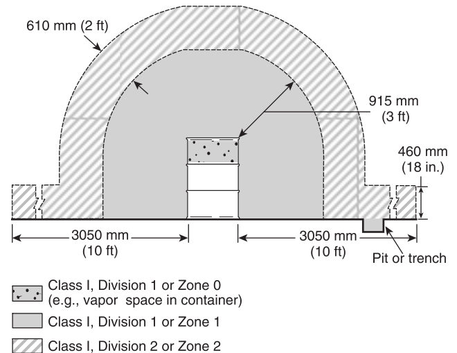
FIGURE 43.1.4.5.2 Electrical Area Classification for Class I Liquid Operations Around Open Containers, Supply Containers, Waste Containers, Spray Gun Cleaners, and Solvent Distillation Units. [33:Figure 6.5.5.2]
