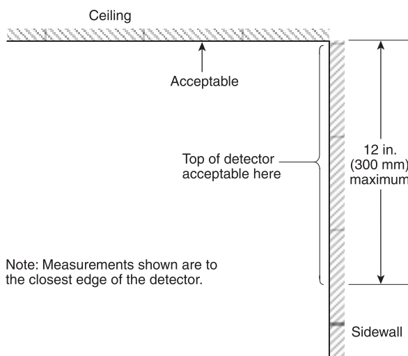
Δ FIGURE A.13.7.4.3.3.1 Example of Proper Mounting of Smoke Detectors. [72: Figure A.17.7.4.2.1]
