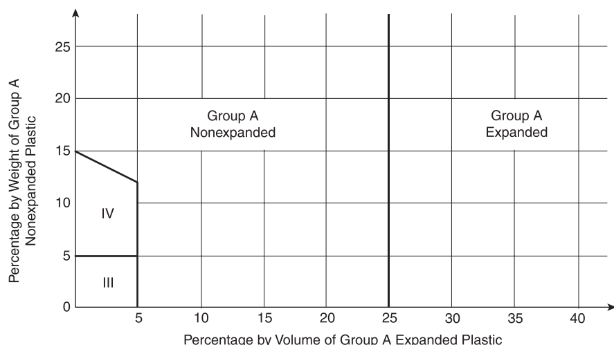
FIGURE 34.3.3.3(b) Exposed Commodities Containing a Mixture of Expanded and Nonexpanded Group A Plastics. [13:Figure 20.4.3.3(b)]
