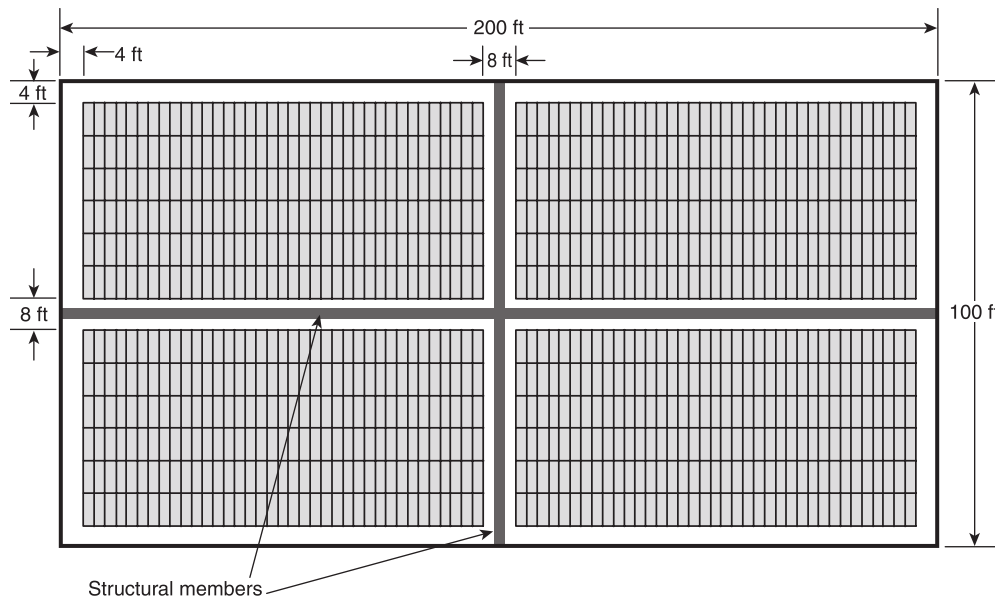
FIGURE A.11.12.3.4.2(1) Commercial Array with an Axis Less Than 250 ft (76.2 m) and with 8 ft (2.4 m) Walkways. (Source: Cal Fire.)
